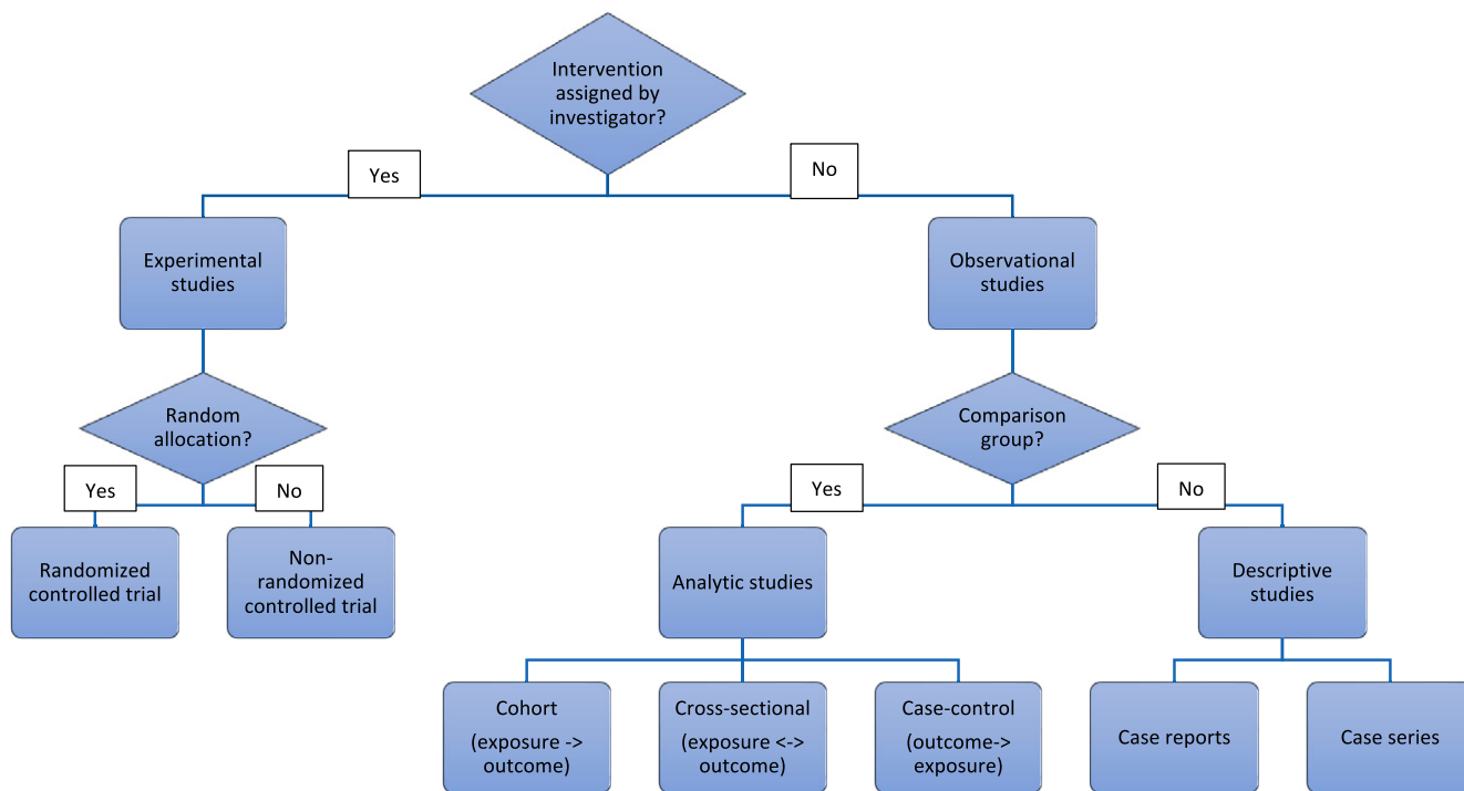
SUPPLEMENTAL FIGURE 1 Organizational chart of quantitative study designs in clinical research.
